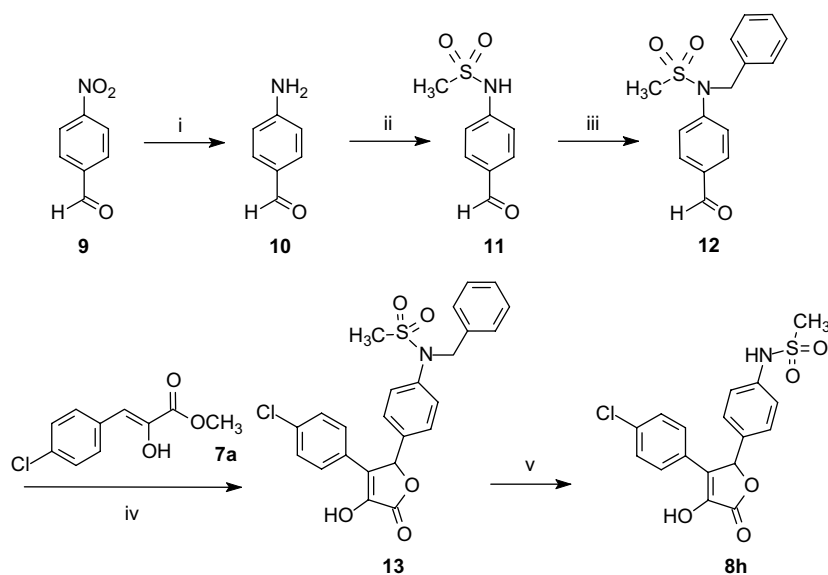
Scheme 2. Reagents and conditions: (i) \text{SnCl}_2 , \text{EtOH} ; (ii) \text{CH}_3\text{SO}_2\text{Cl} , pyridine; (iii) \text{BnCl} , \text{NEt}_3 , \text{DMF} , 80^\circ\text{C} ; (iv) \text{DBU} , \text{DMF} , 0^\circ\text{C} ; (v) \text{Pd/C} , \text{H}_2 , \text{THF/EtOH} .
