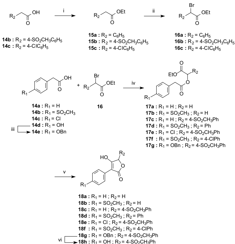
Scheme 3. Reagents and conditions: (i) DBU, \text{CH}_3\text{CH}_2\text{I} , DMF, 0^\circ\text{C} ; (ii) NBS, (\text{PhCOO})_2 , \text{CCl}_4 , reflux; (iii) \text{BnCl} , \text{K}_2\text{CO}_3 , KI, DMF, reflux; (iv) \text{NEt}_3 , THF, reflux; (v) NaH, THF; (vi) Pd/C, \text{H}_2 , THF/EtOH.
