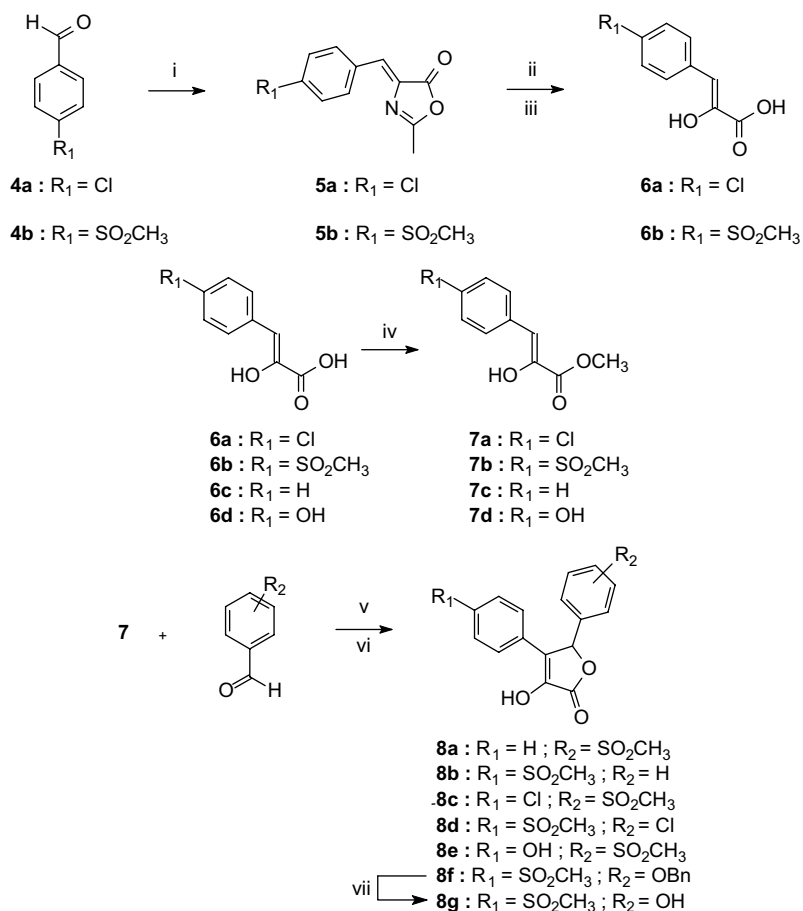
Scheme 1. Reagents and conditions: (i) N -acetylglycine, \text{Ac}_2\text{O} , \text{AcONa} , 100^\circ\text{C} ; (ii) \text{NaOH} ; (iii) \text{HCl} , reflux; (iv) \text{DBU} , \text{CH}_3\text{I} , \text{DMF} , 0^\circ\text{C} ; (v) \text{DBU} , \text{DMF} , 0^\circ\text{C} ; (vi) \text{HCl} ; (vii) \text{Pd/C} , \text{H}_2 , \text{THF/EtOH} .
